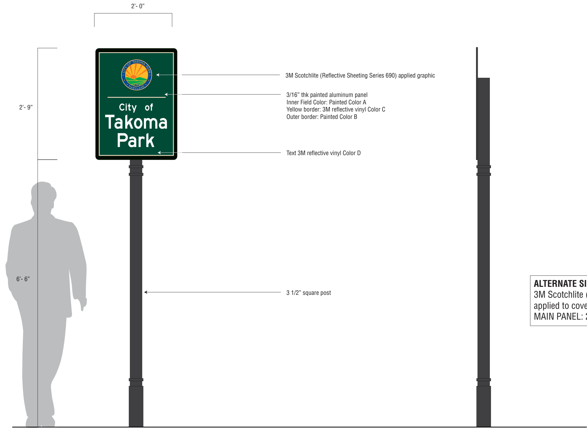
1 SIGN TYPE A.2 - SECONDARY GATEWAY FRONT VIEW
